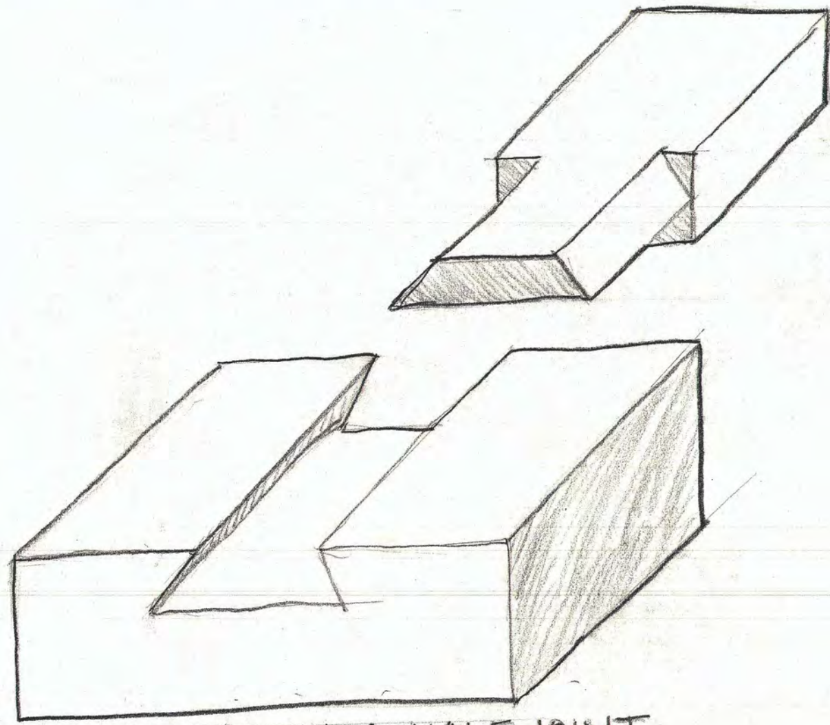
DOVETAILED & HALF JOINT
