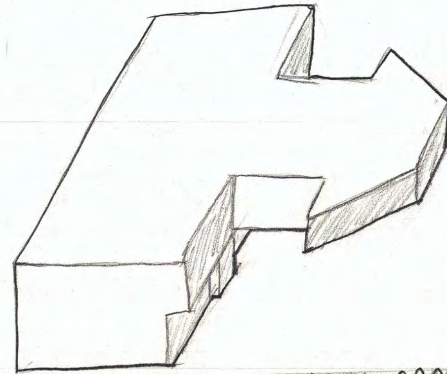
STEPPED GOOSENECK SPLICE
